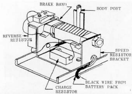
Diagram showing additional wiring for reverse kit. On right is standard resistor rig. Microswitch for reverse is screwed into two holes seen on left if desired.
