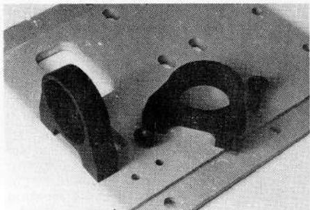
These are the smart anodised alloy plummer blocks that save weight and reduce CG slightly.
